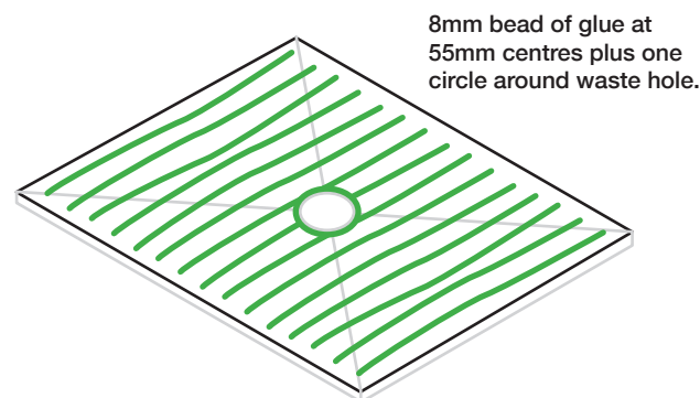
Diagram 2: Bonding of Tray - Underside view
